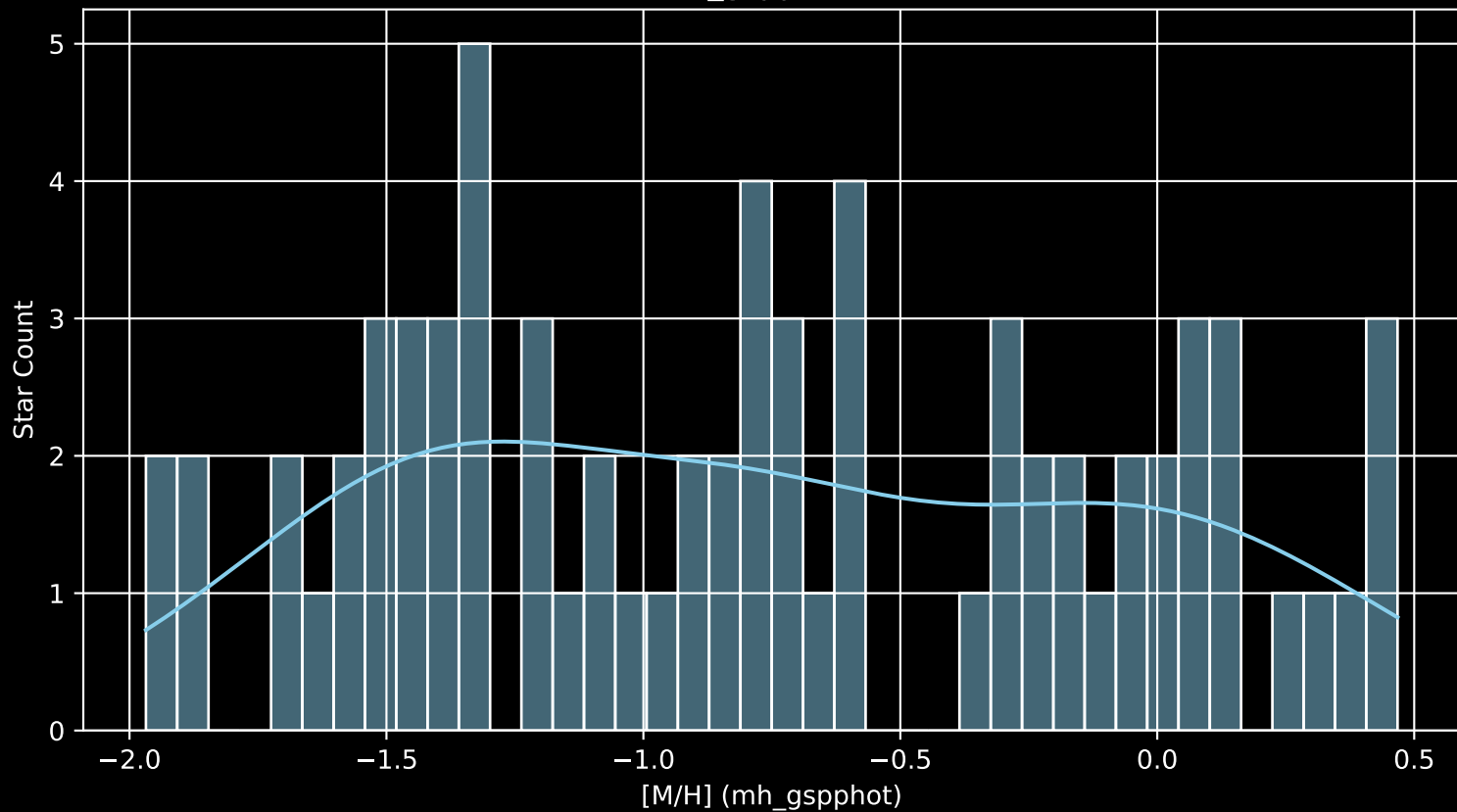
APOGEE DR17 Field: [000+02-O [M/H] (mh_gspphot) (n= 72)
