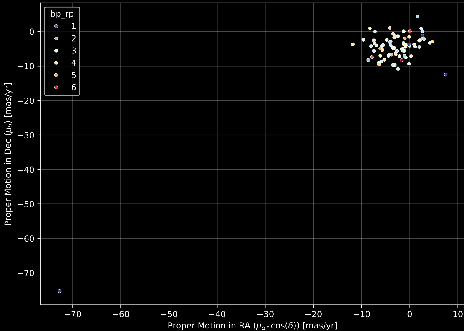
APOGEE DR17 Field: [000+02-O] Proper Motion Diagram (n= 76)
