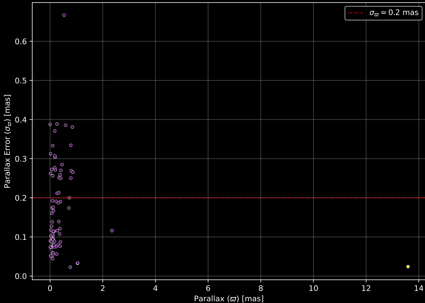
APOGEE DR17 Field: [000+02-O] Parallax Quality (n= 76)
