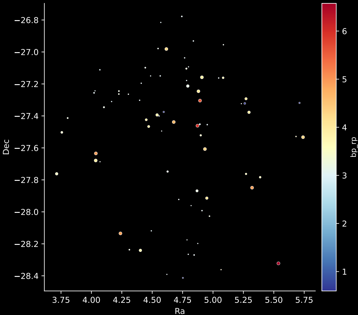
APOGEE DR17 Field: [000+02-O] Stars: 76
