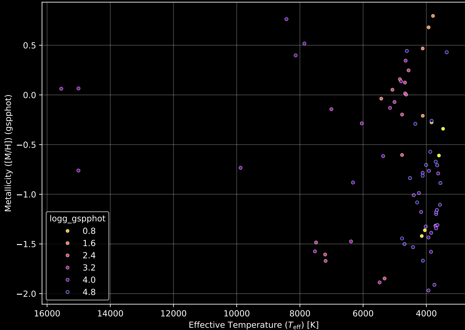
APOGEE DR17 Field: [000+02-O] Stellar Population Parameters (n= 76)
